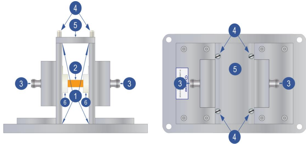
Figure 2 – FCLCE-452 Calibration Fixture Features
