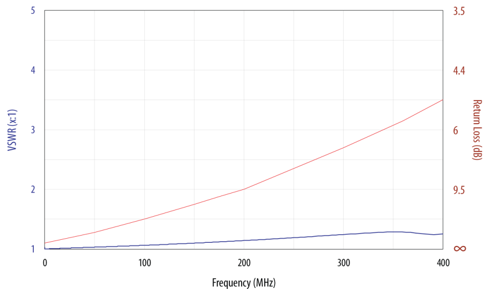
Figure 6 – Typical VSWR/Return Loss for FCLCE-452 Calibration Fixture
