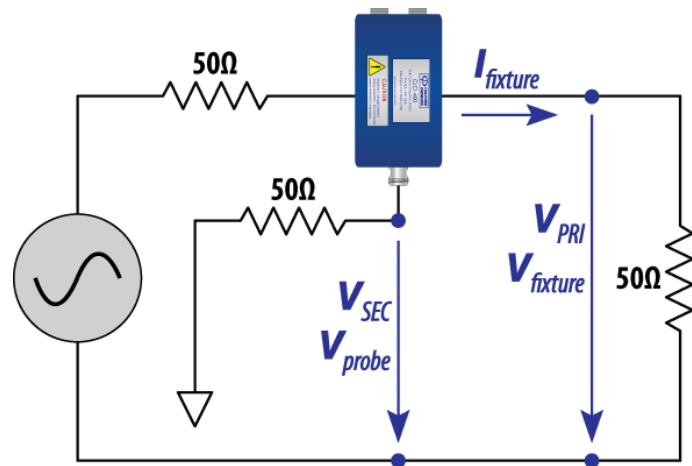
Figure 9 – Equivalent Schematics of the Insertion Loss Calibration Circuits
