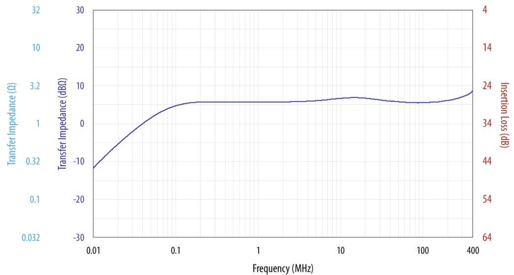
Figure 5 – Typical Insertion Loss/Transfer Impedance Factors for CLCE-452 Probe
