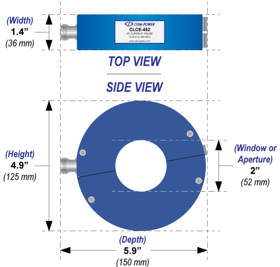
Figure 3 – CLCE-452 RF Current Probe Dimensions
