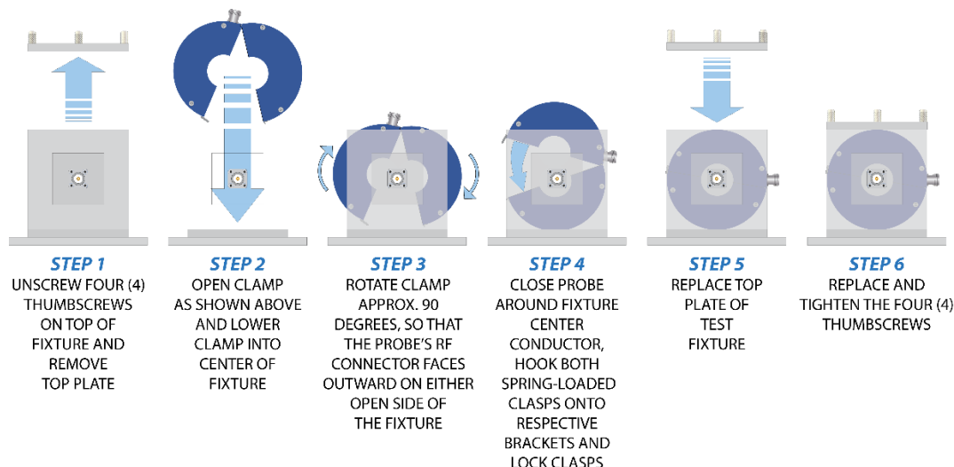
Figure 8 – Installation of CLCE-452 Probe into FCLCE-452 Fixture
