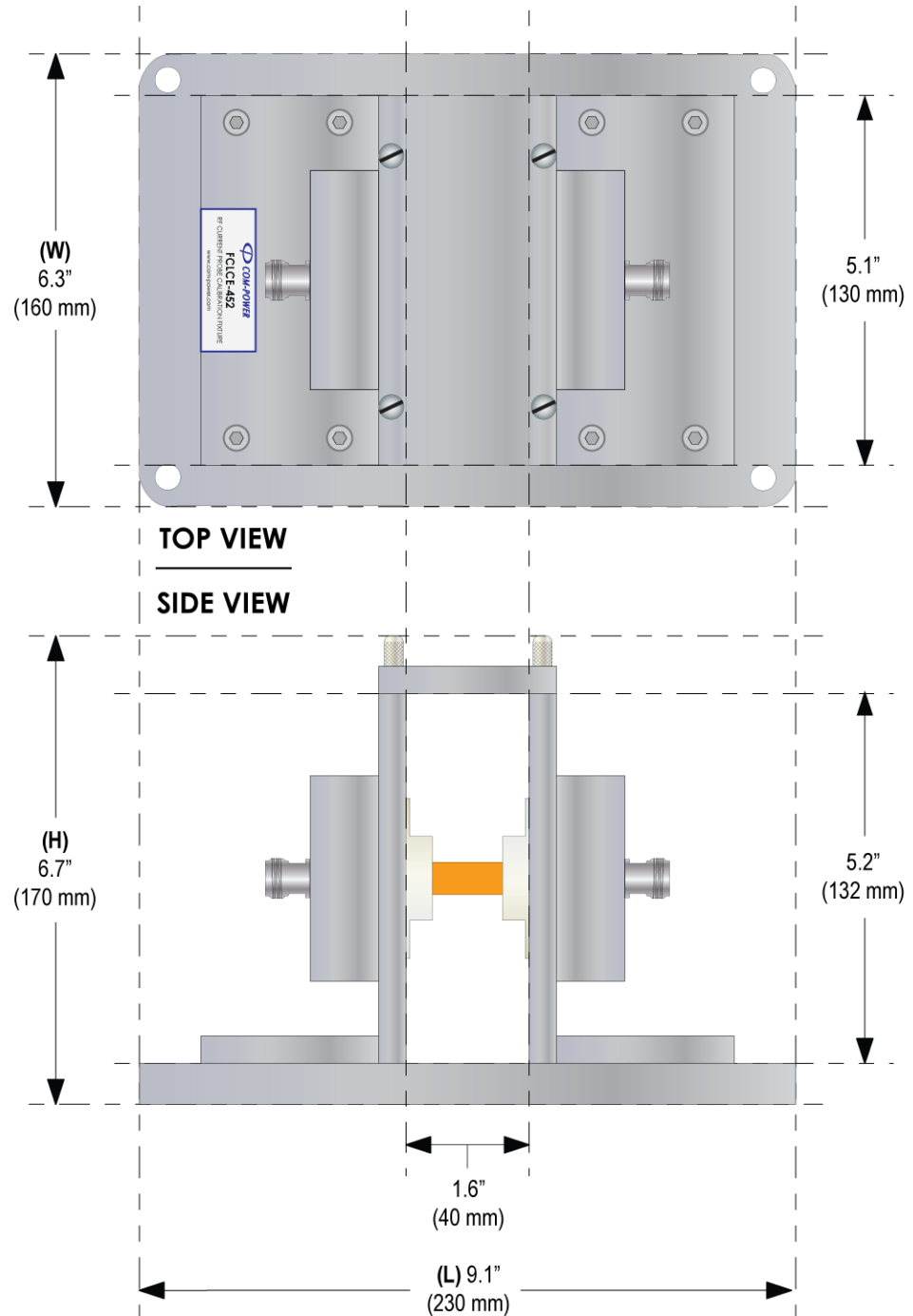
Figure 4 – FCLCE-452 Calibration Fixture Dimensions
