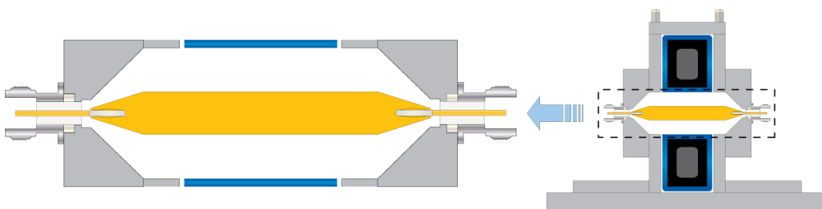
Figure 7 – Cross-Sectional Diagram of Calibration Fixture with Probe Installed
