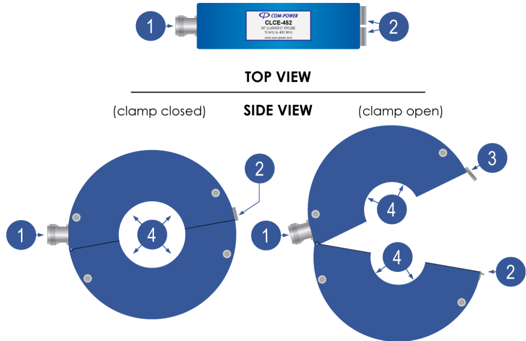
Figure 1 – CLCE-452 RF Current Probe Features
