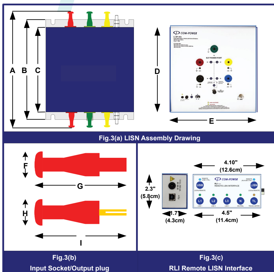
FIGURE 3 - Product Dimensions
