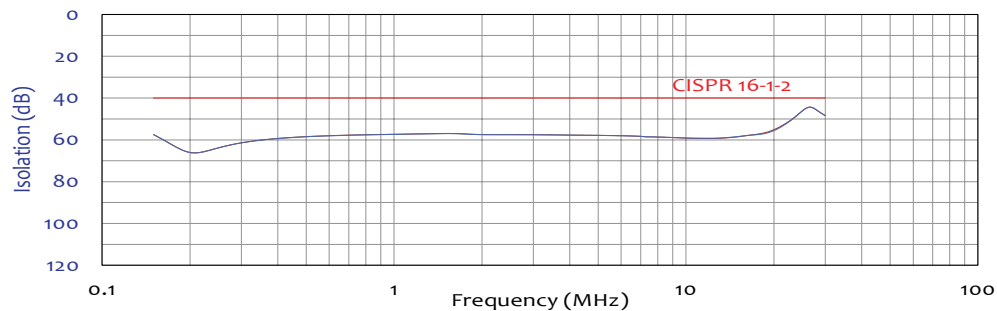
FIGURE 4 - Product Performance Data
