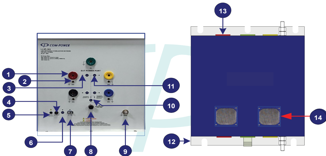
FIGURE 1 - Product Features – Front Panel and Top View
