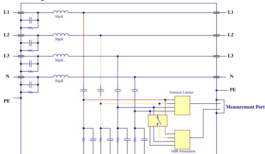
FIGURE 5 – Schematic Diagram of LI-3P-1100
