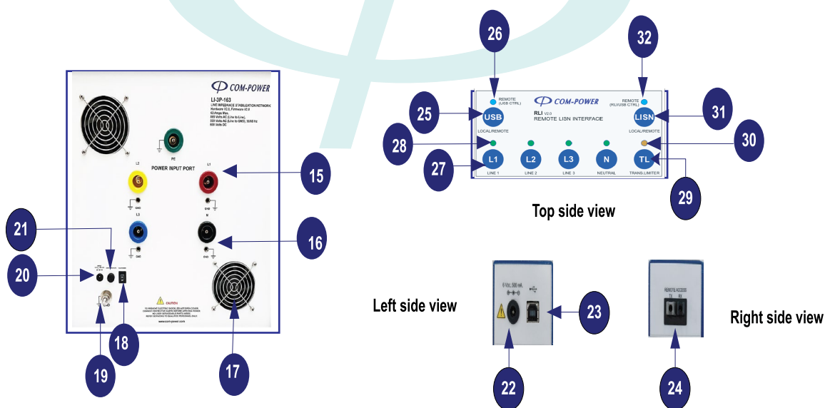
FIGURE 2 - Product Features – Rear Panel & RLI V2.0
