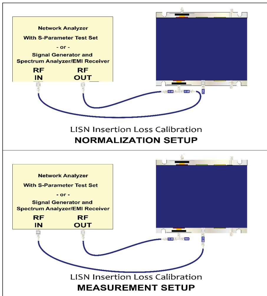
FIGURE 11 – Setup Diagrams for LISN Insertion Loss Calibration
