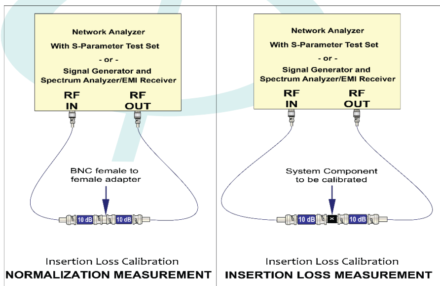
FIGURE 12 – Setup Diagrams for Non-LISN Insertion Loss Calibration
