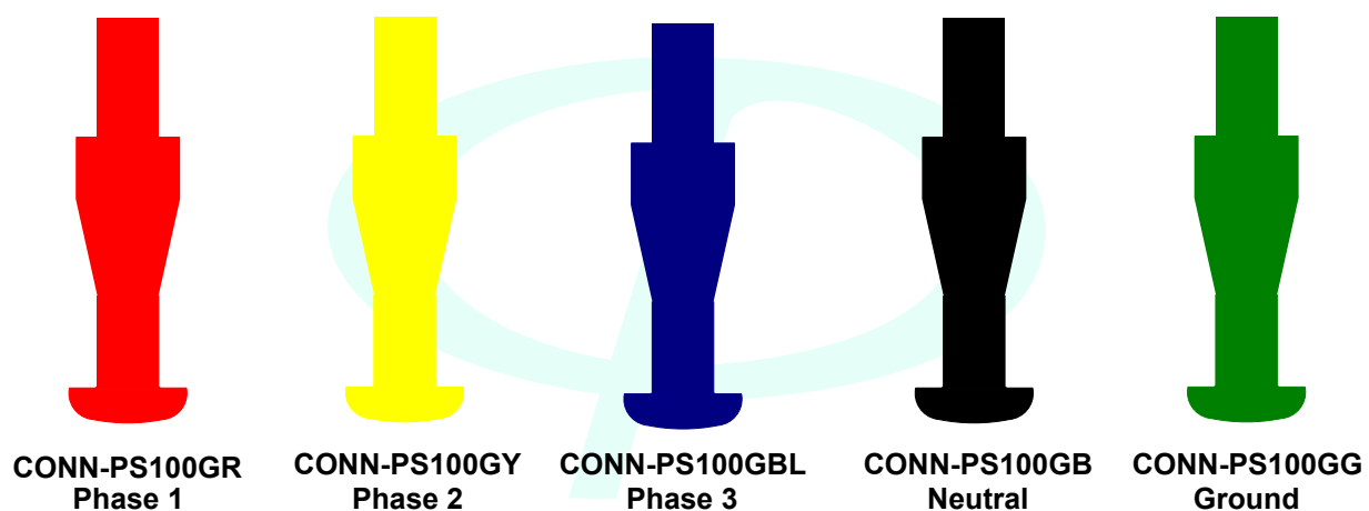
FIGURE 7 – Power Input Port Plug Socket Connectors (100 Ampere)
