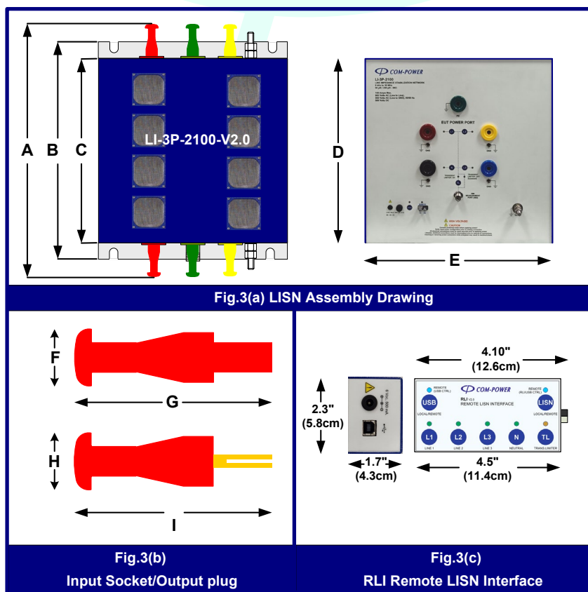
FIGURE 3 - Product Dimensions SECTION 3 - PRODUCT INFORMATION
