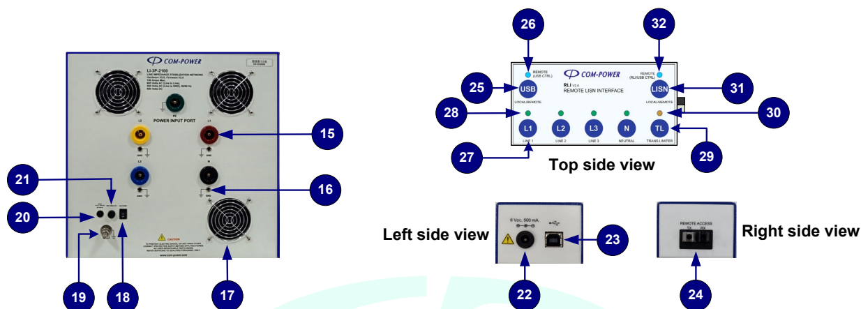
FIGURE 2 - Product Features – Rear Panel & RLI v2.0
