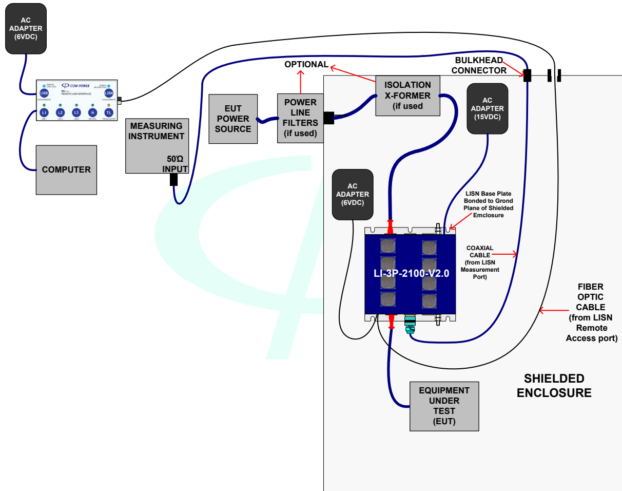
FIGURE 6 – Typical Test Setup
