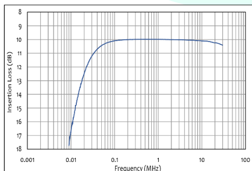
Typical Insertion Loss Data
