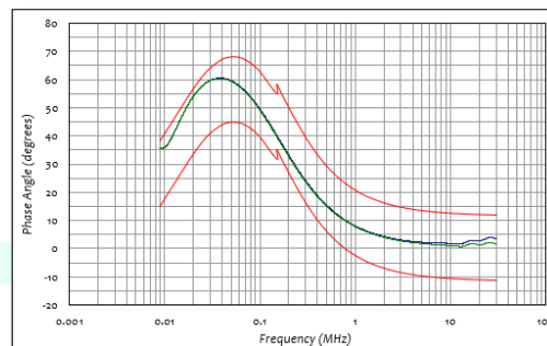
Typical Phase Data
