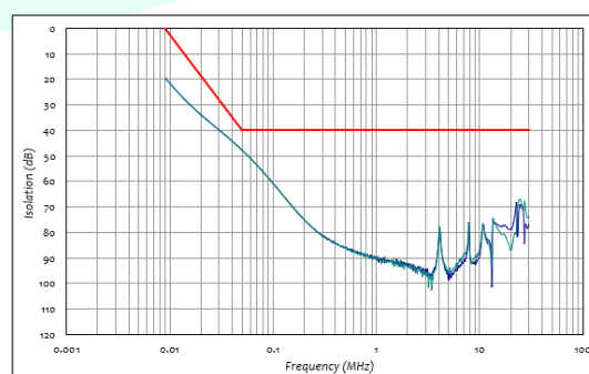
Typical Isolation Data
