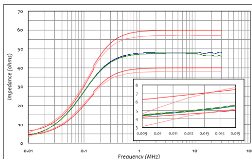
Typical Impedance Data
