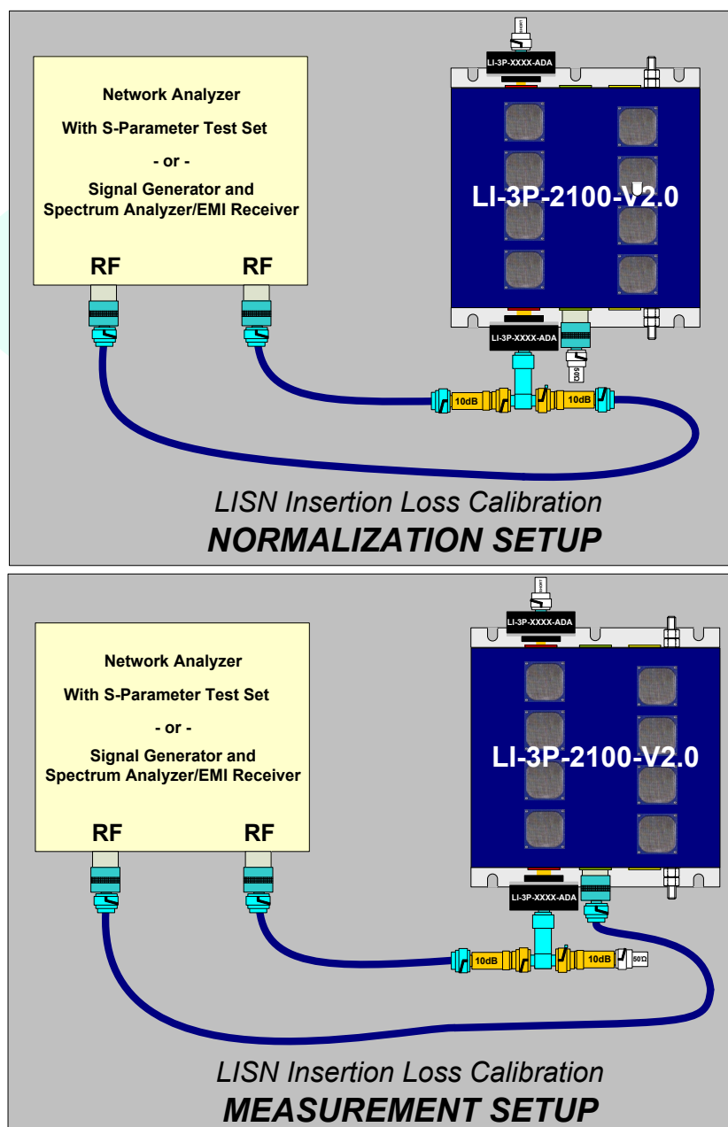
FIGURE 11 – Setup Diagrams for LISN Insertion Loss Calibration SECTION 6 – LISN MEASUREMENTS
