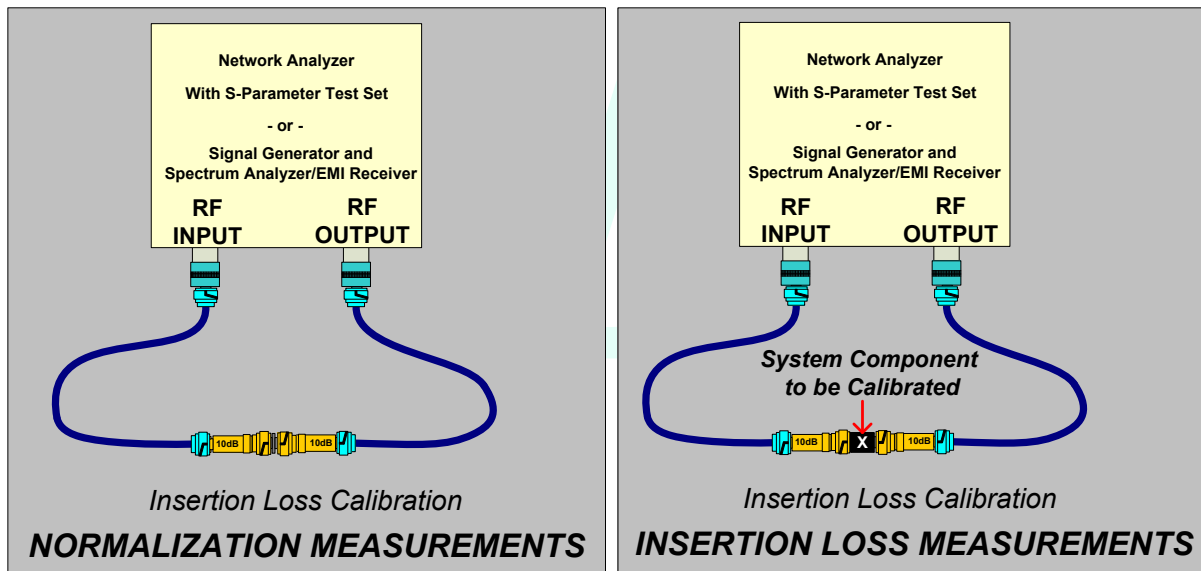
FIGURE 12 – Setup Diagrams for Insertion Loss Calibration
