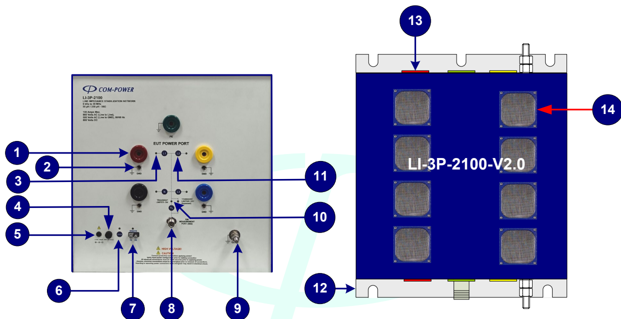
FIGURE 1 - Product Features – Front Panel and Top View
