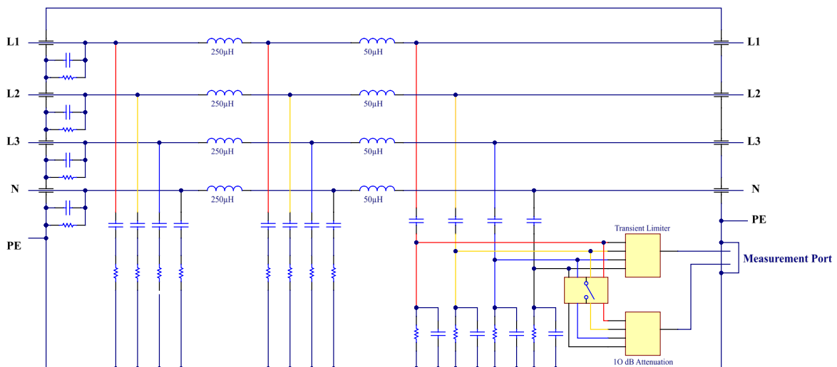
FIGURE 5 – Schematic Diagram of LI-3P-2100
