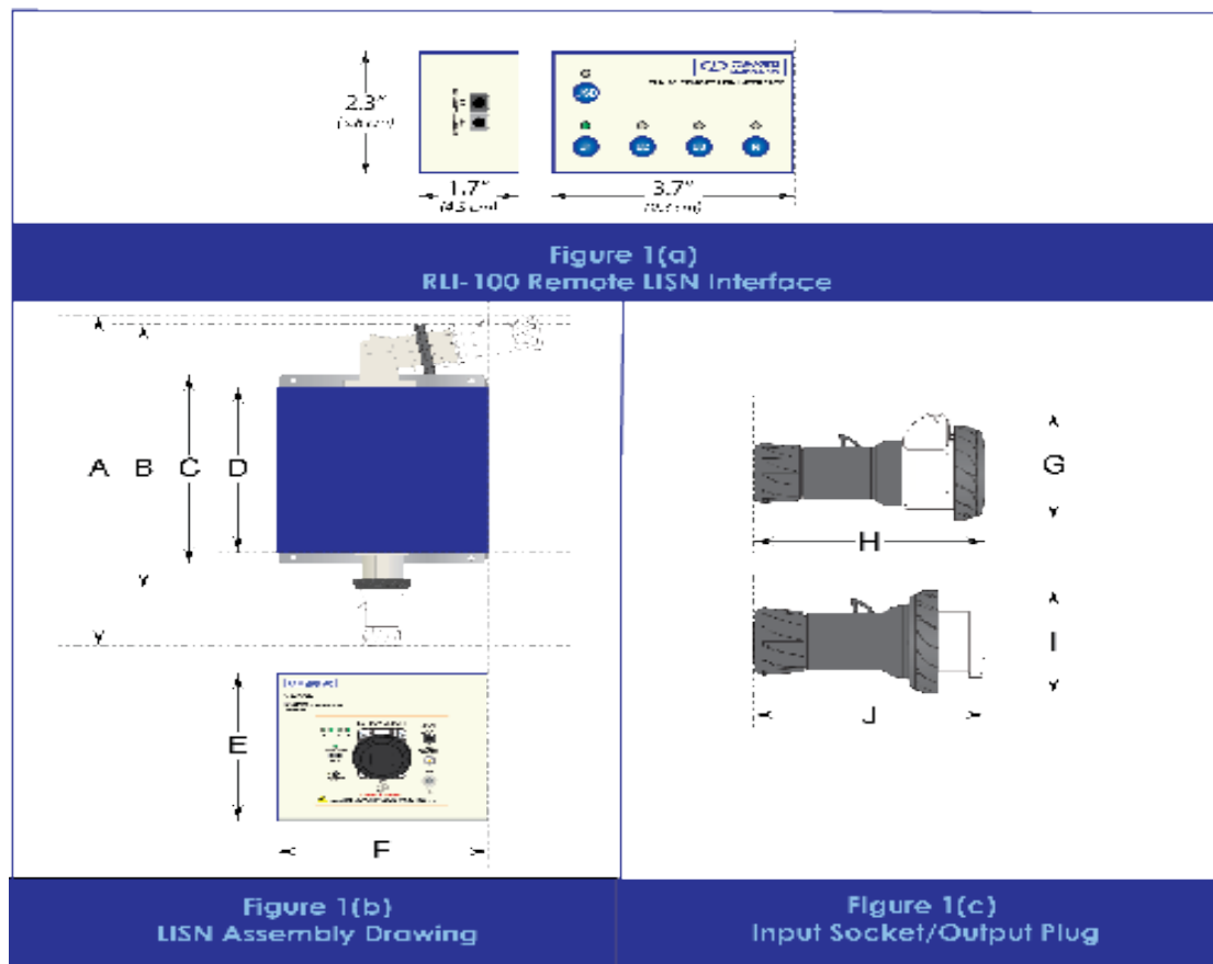
Figure 1 - Product Dimensions
