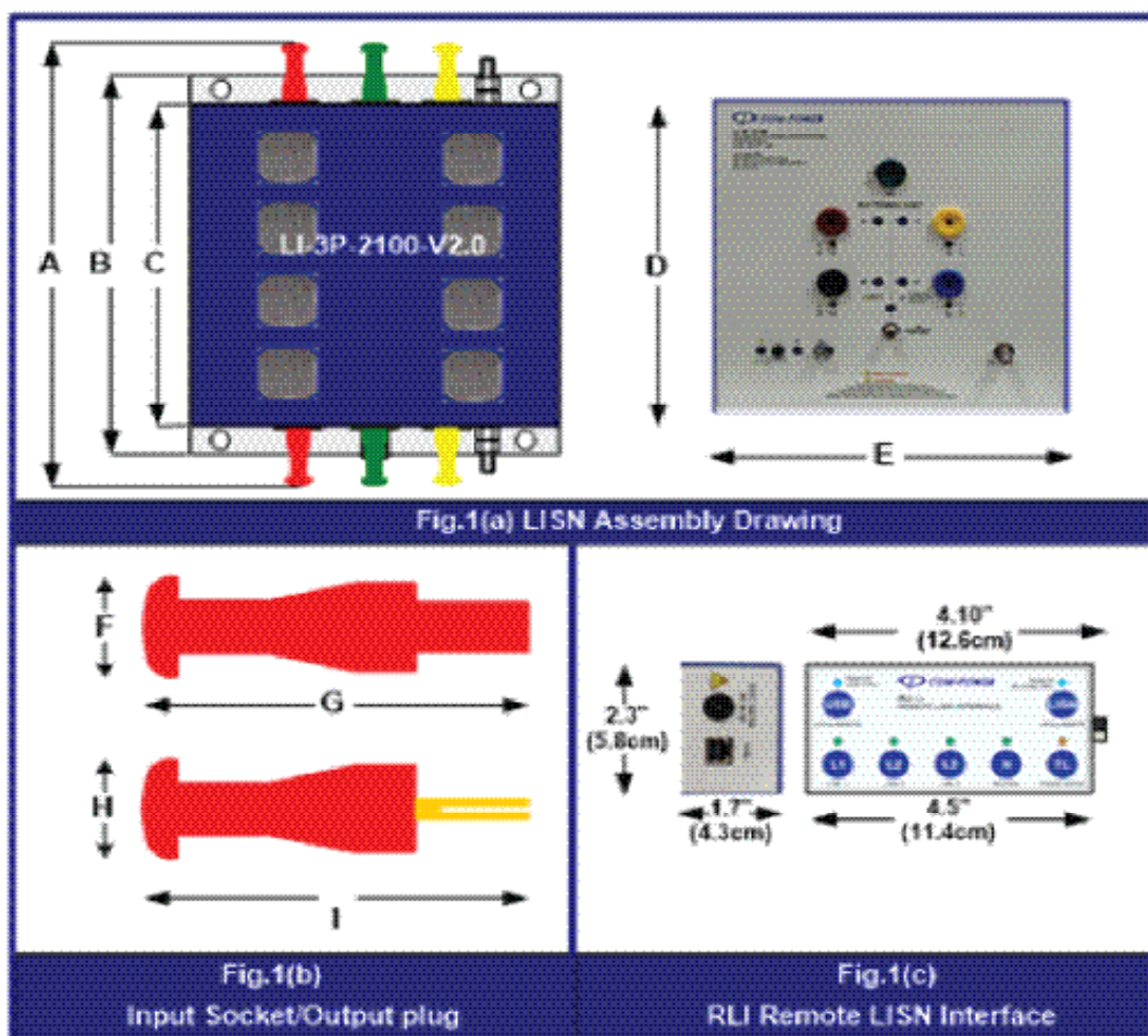
Figure 1 - Product Dimensions
